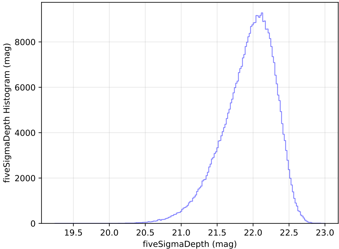
weather_cloudso35v3.4_10yrs y: fiveSigmaDepth Histogram
