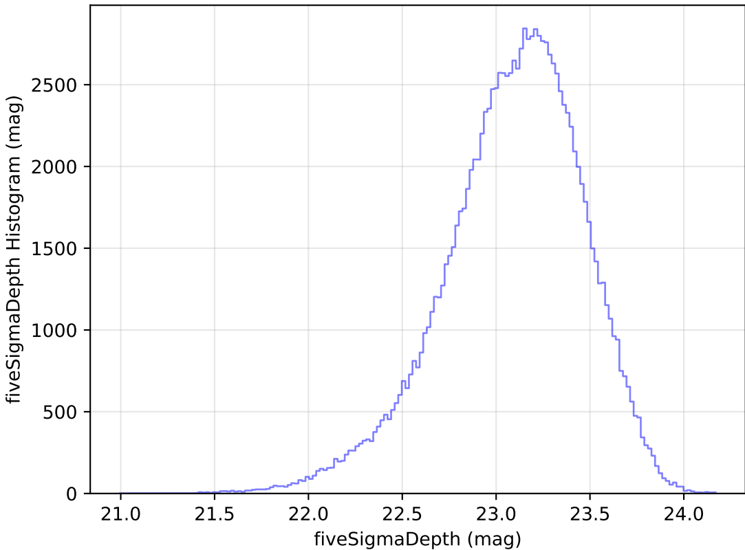
weather_cloudso35v3.4_10yrs u: fiveSigmaDepth Histogram
