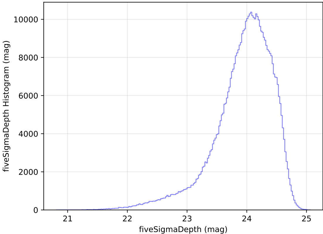
weather_cloudso35v3.4_10yrs r: fiveSigmaDepth Histogram
