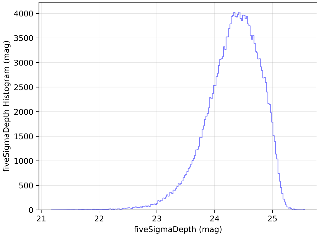
weather_cloudso35v3.4_10yrs g: fiveSigmaDepth Histogram
