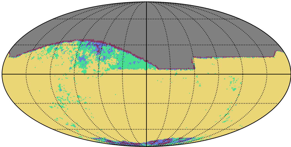
weather_cloudso35v3.4_10yrs z band: YearCoverage night
