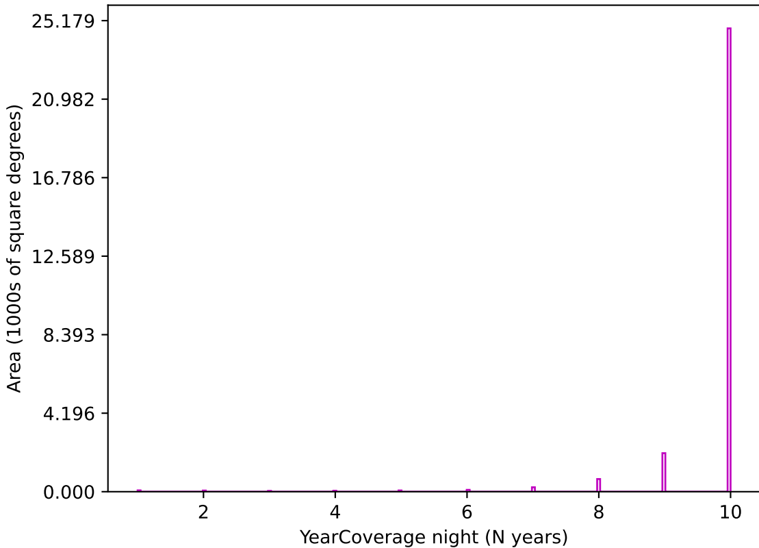
weather_cloudso35v3.4_10yrs z band: YearCoverage night
