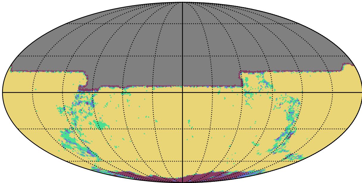
weather_cloudso35v3.4_10yrs y band: YearCoverage night
