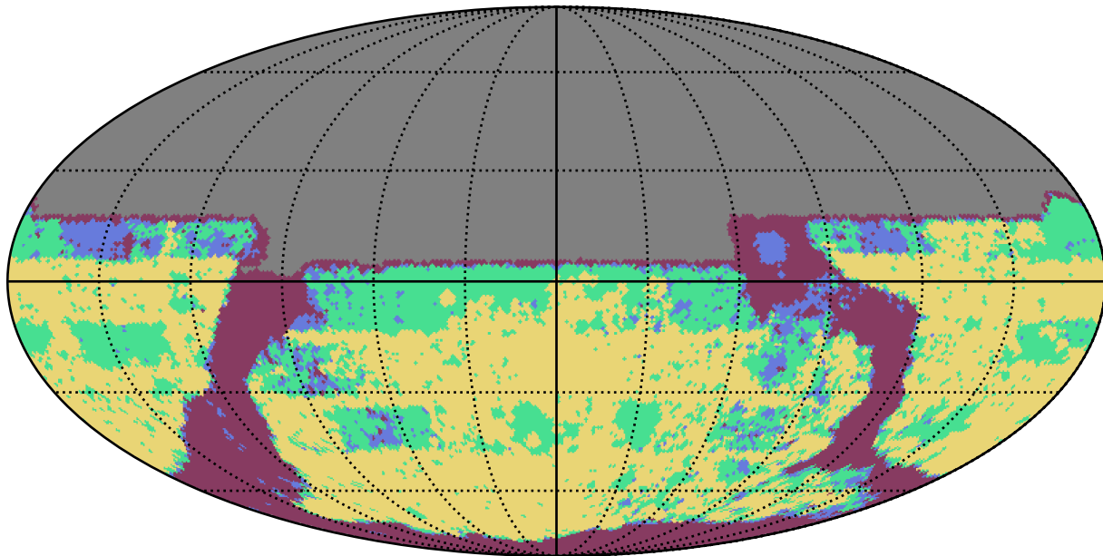
weather_cloudso35v3.4_10yrs u band: YearCoverage night
