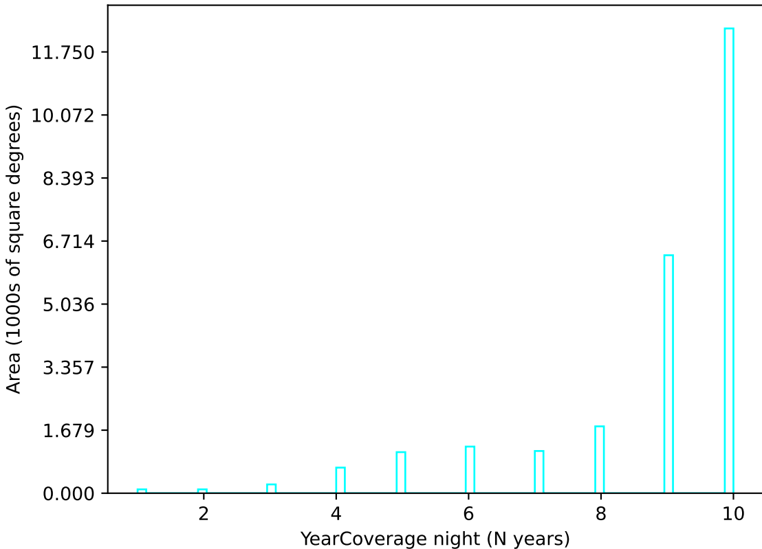
weather_cloudso35v3.4_10yrs u band: YearCoverage night
