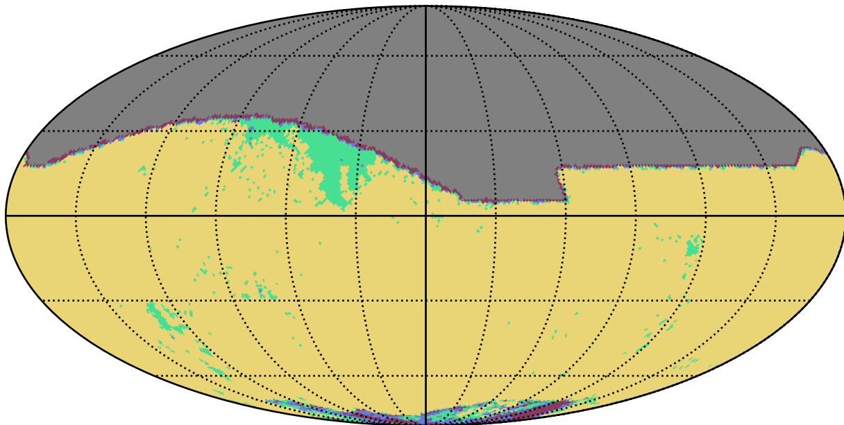
weather_cloudso35v3.4_10yrs r band: YearCoverage night
