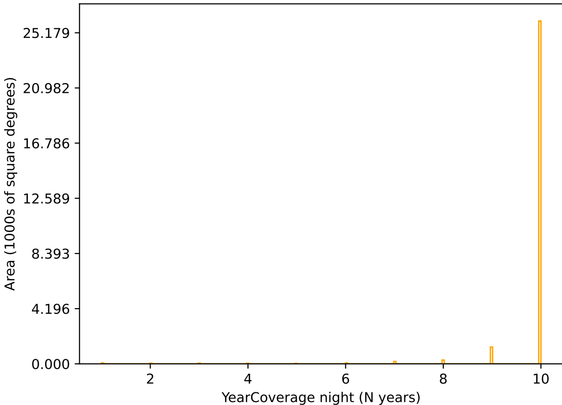
weather_cloudso35v3.4_10yrs r band: YearCoverage night
