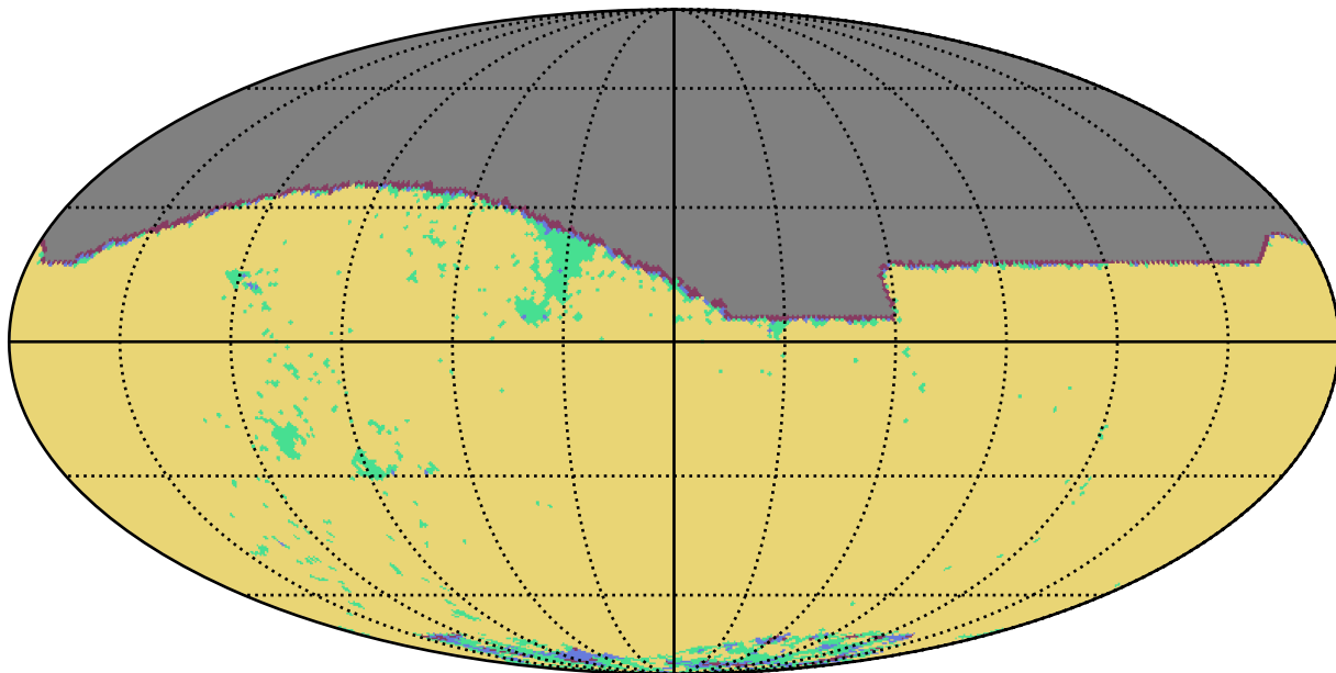
weather_cloudso35v3.4_10yrs i band: YearCoverage night
