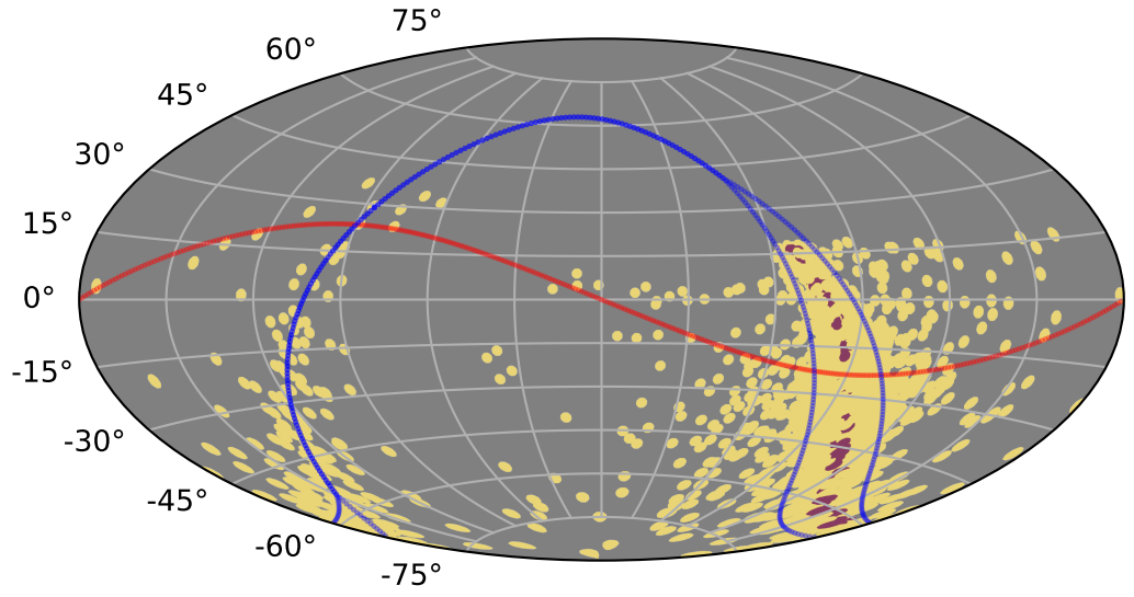
weather_cloudso35v3.4_10yrs : XRBPpopMetric_possible_to_detect
