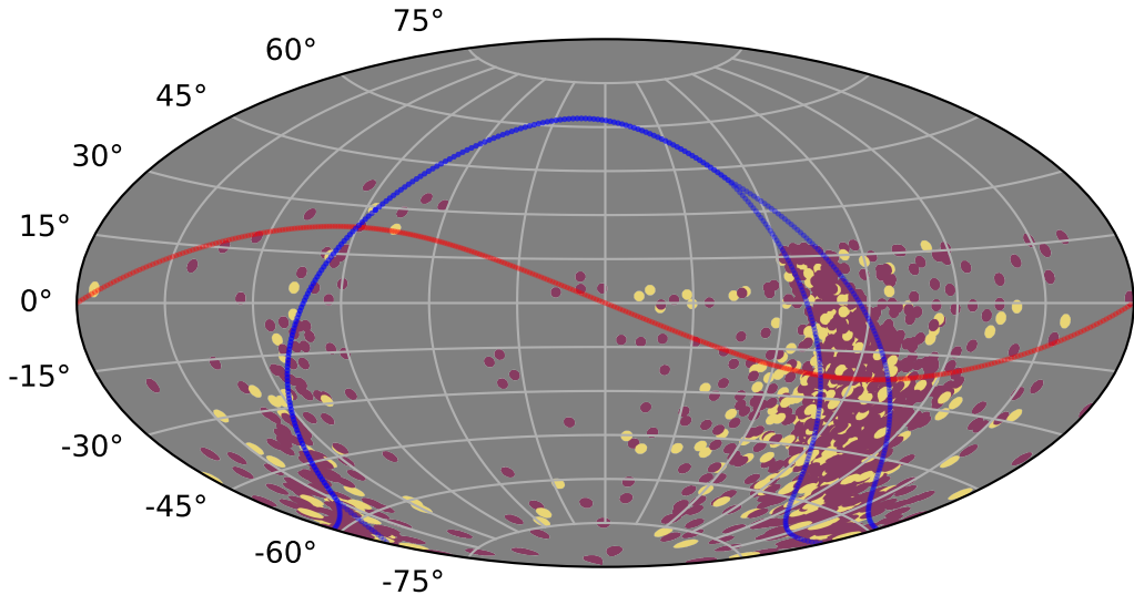
weather_cloudso35v3.4_10yrs : XRBPoPMetric_early_detect
