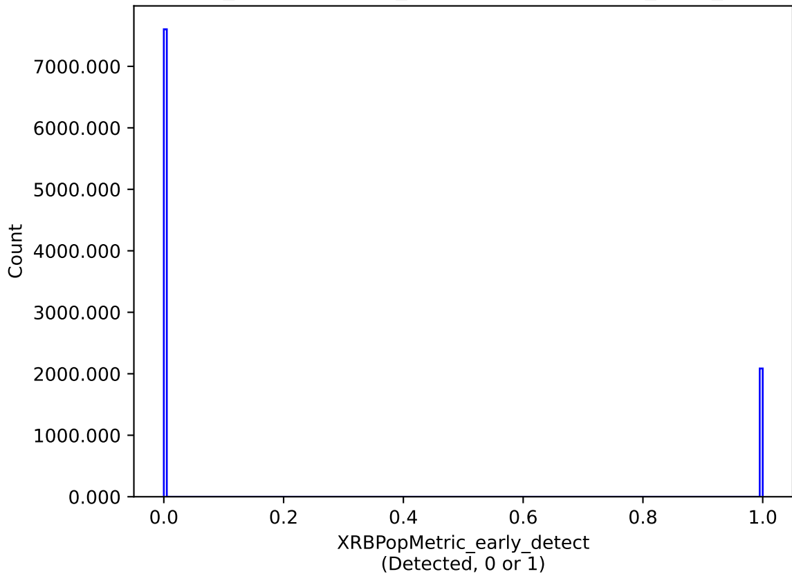
weather_cloudso35v3.4_10yrs : XRBPoMetric_early_detect
