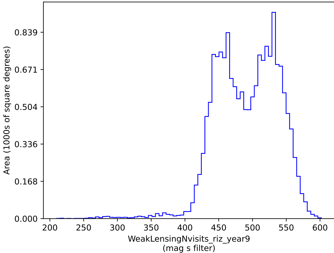
weather_cloudso35v3.4_10yrs gri band non-DD: WeakLensingNvisits_riz_year9
