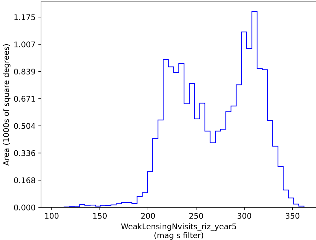
weather_cloudso35v3.4_10yrs gri band non-DD: WeakLensingNvisits_riz_year5
