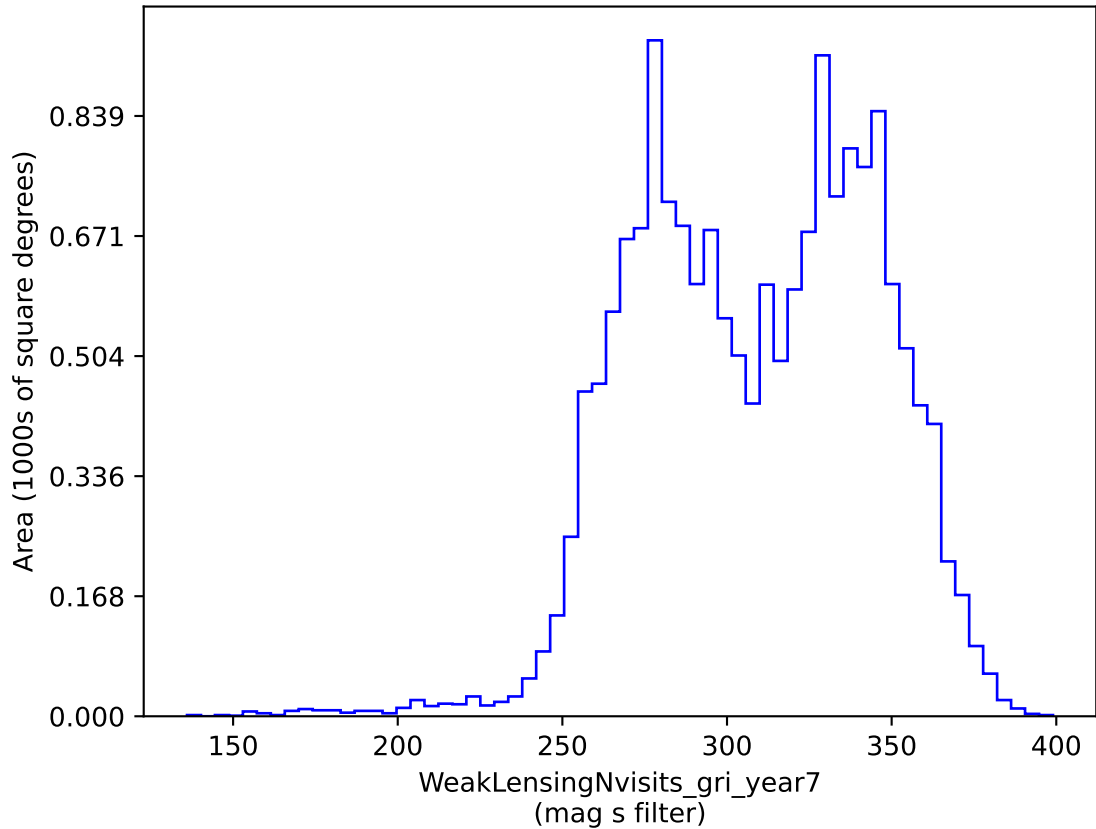
weather_cloudso35v3.4_10yrs gri band non-DD: WeakLensingNvisits_gri_year7
