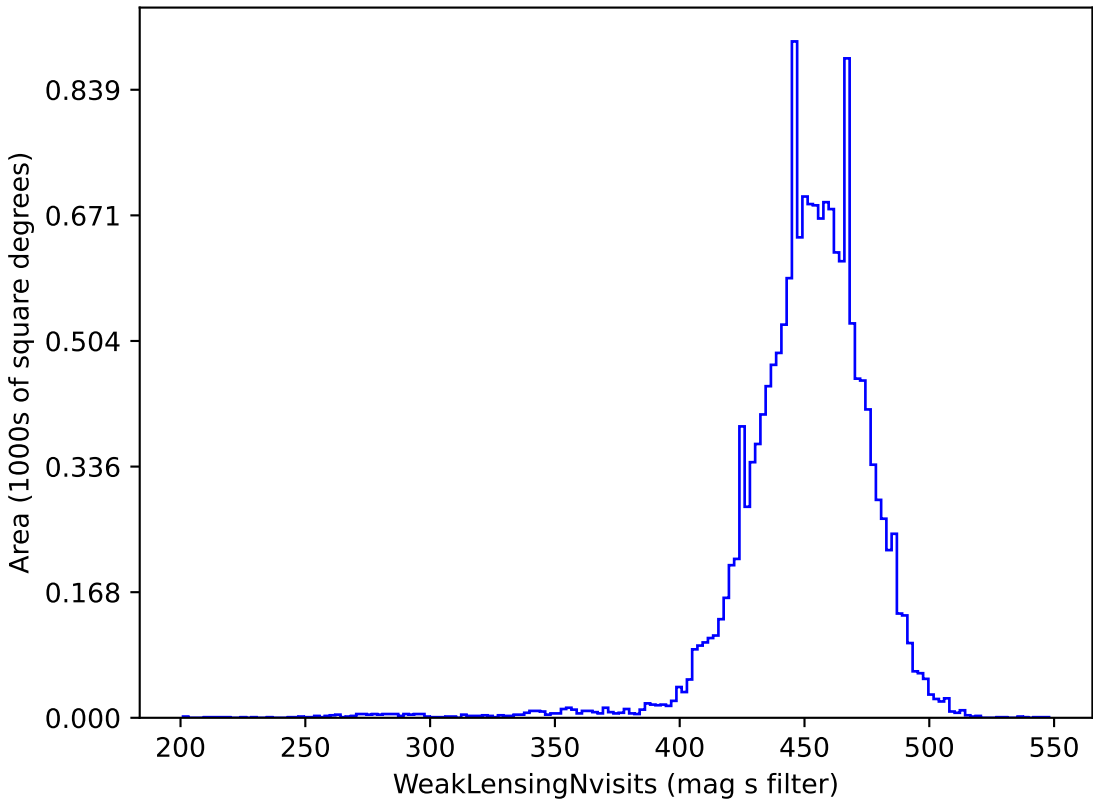
weather_cloudso35v3.4_10yrs gri band non-DD: WeakLensingNvisits
