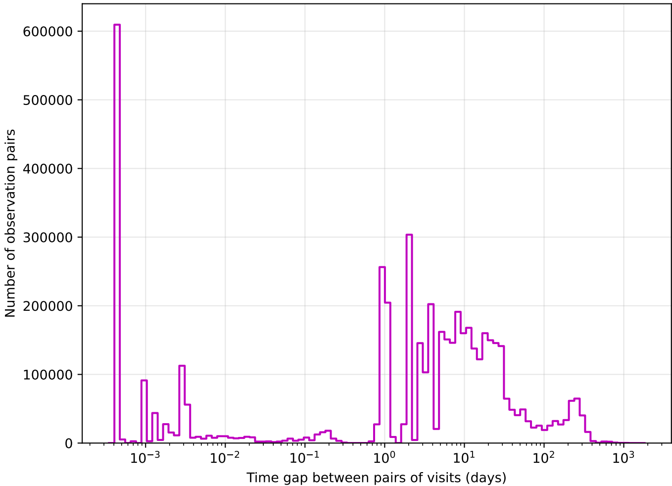
weather_cloudso35v3.4_10yrs z band: Tgaps observationStartMJD
