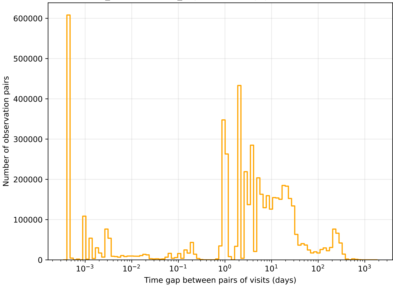
weather_cloudso35v3.4_10yrs r band: Tgaps observationStartMJD
