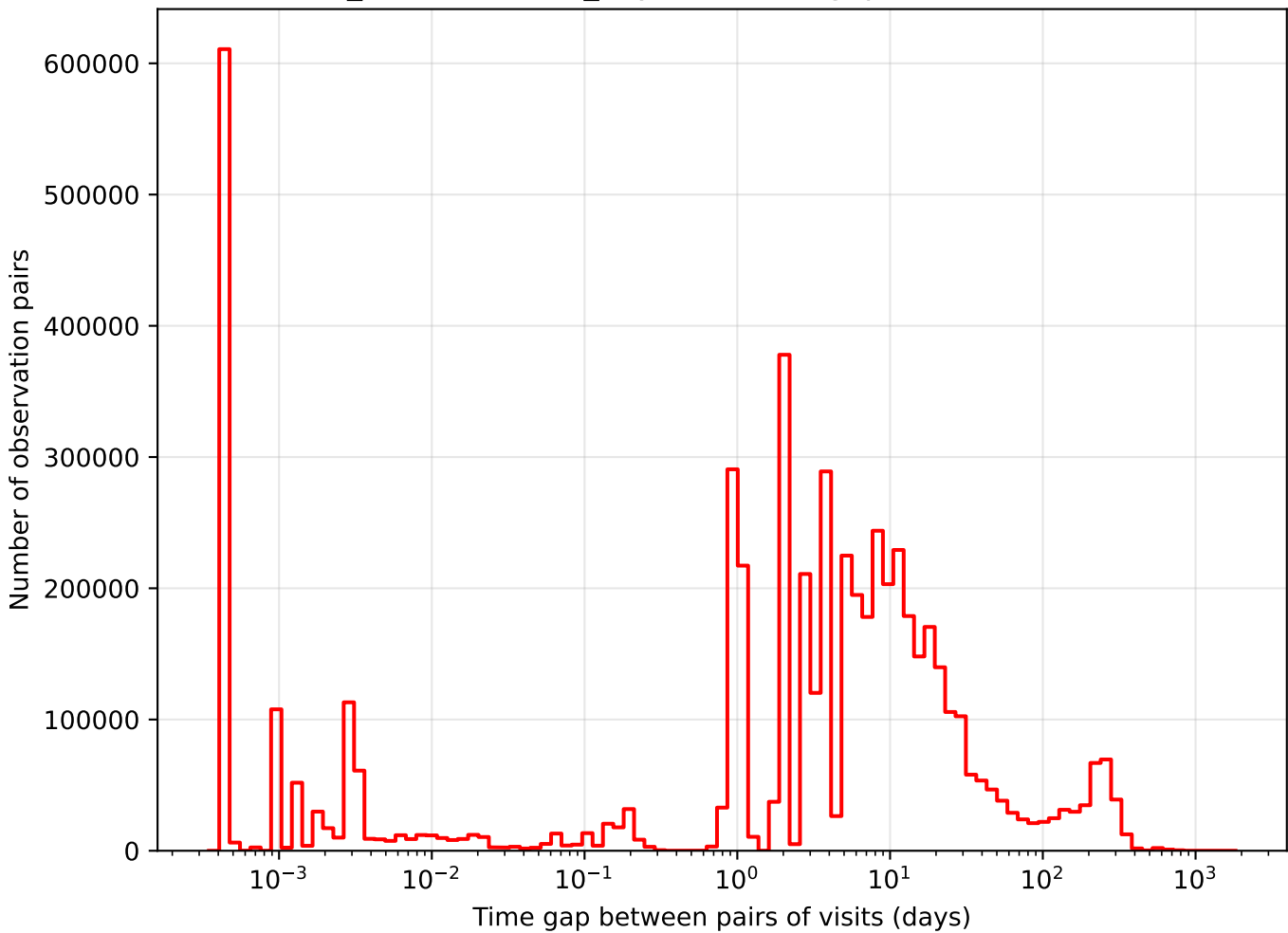
weather_cloudso35v3.4_10yrs i band: Tgaps observationStartMJD
