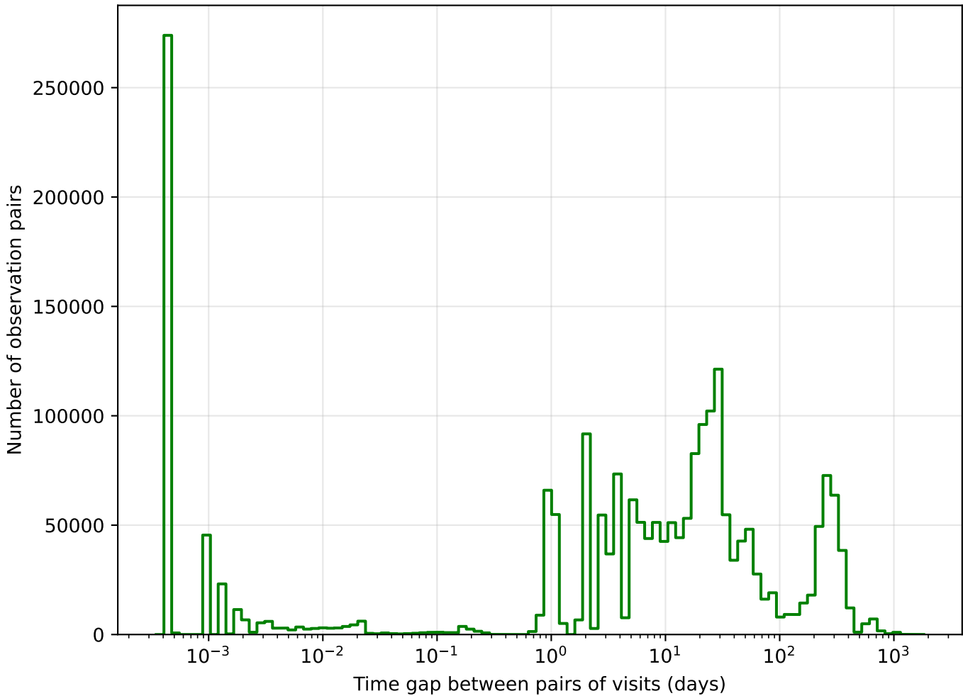
weather_cloudso35v3.4_10yrs g band: Tgaps observationStartMJD
