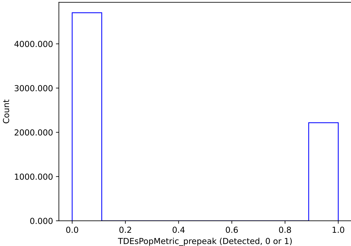
weather_cloudso35v3.4_10yrs : TDEsPopMetric_prepeak
