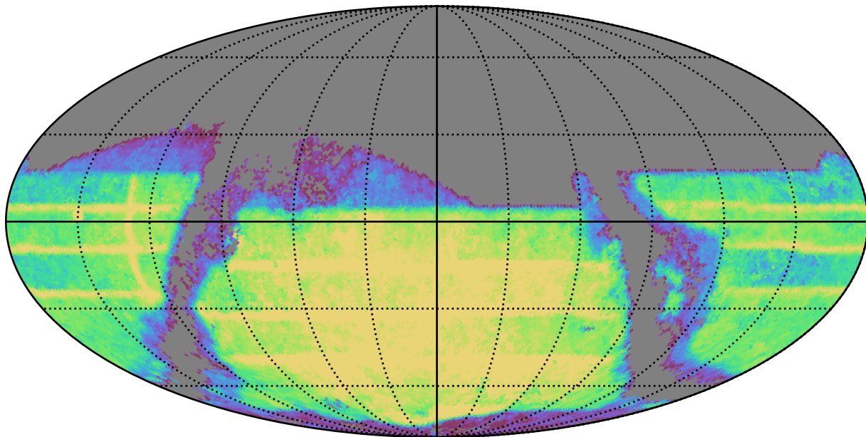
weather_cloudso35v3.4_10yrs : TDC_rate
