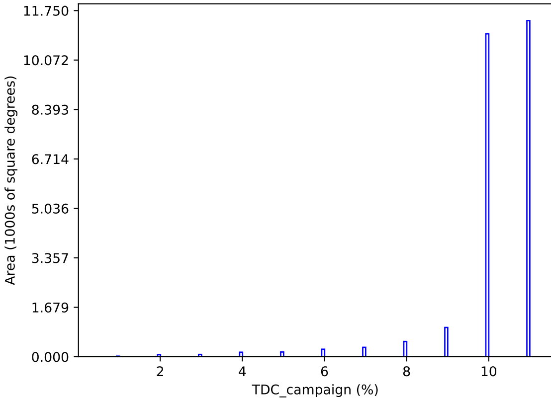
weather_cloudso35v3.4_10yrs : TDC_campaign
