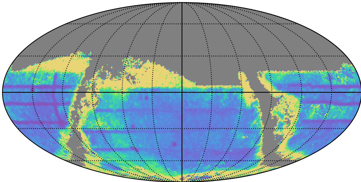
weather_cloudso35v3.4_10yrs : TDC_cadence
