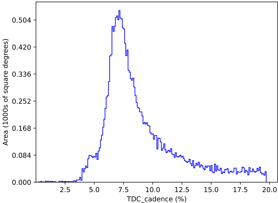
weather_cloudso35v3.4_10yrs : TDC_cadence
