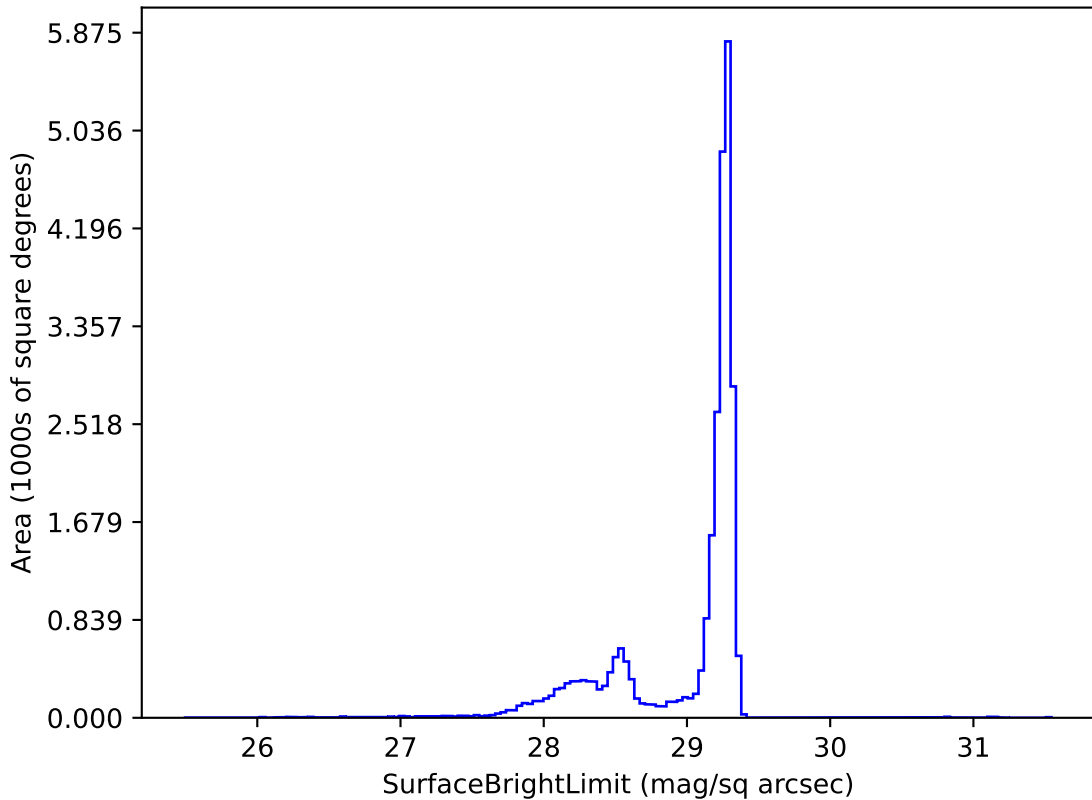
weather_cloudso35v3.4_10yrs z: SurfaceBrightLimit
