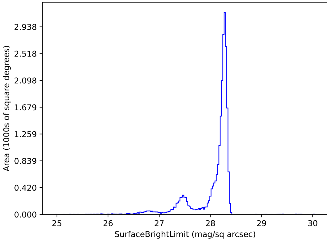
weather_cloudso35v3.4_10yrs y: SurfaceBrightLimit
