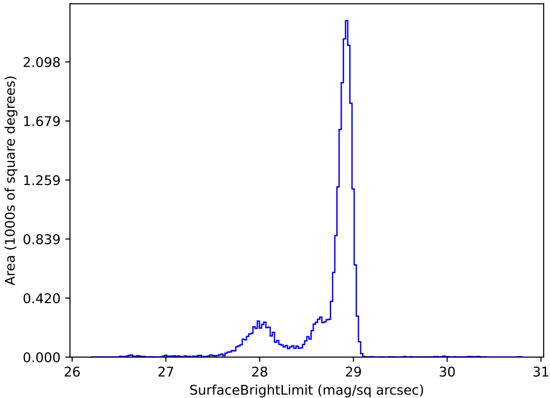
weather_cloudso35v3.4_10yrs u: SurfaceBrightLimit
