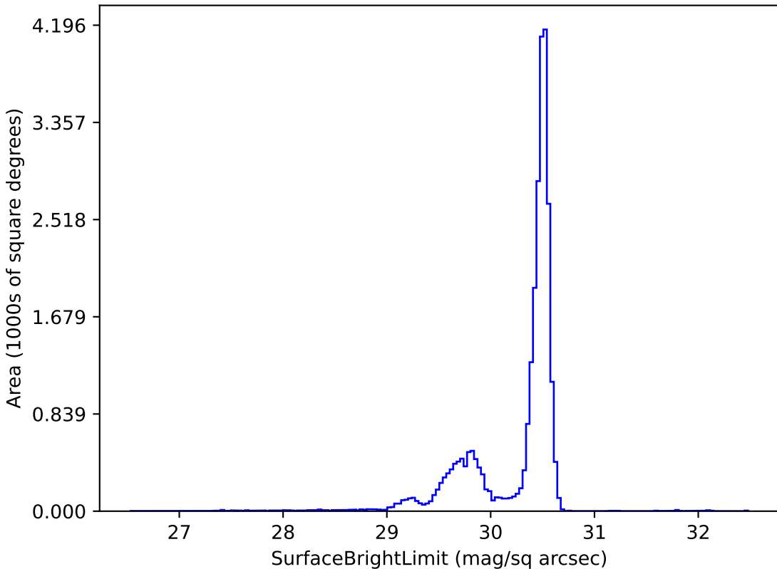
weather_cloudso35v3.4_10yrs r: SurfaceBrightLimit
