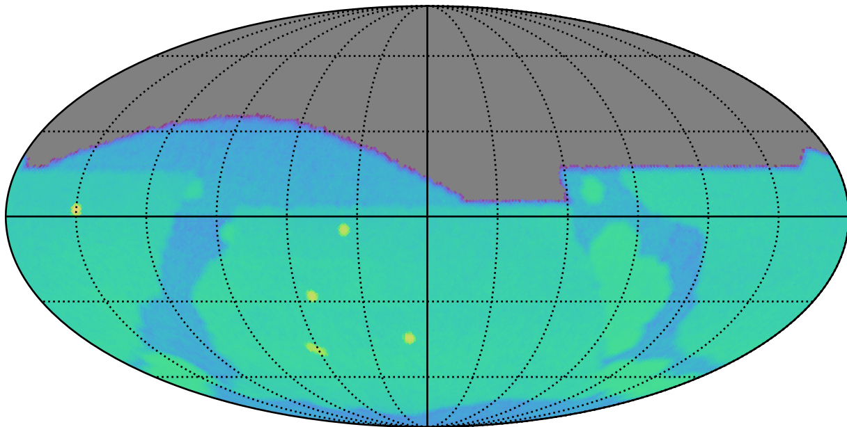
weather_cloudso35v3.4_10yrs g: SurfaceBrightLimit
