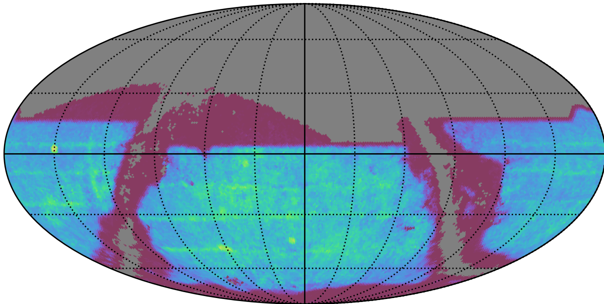
weather_cloudso35v3.4_10yrs : SNSLMetric
