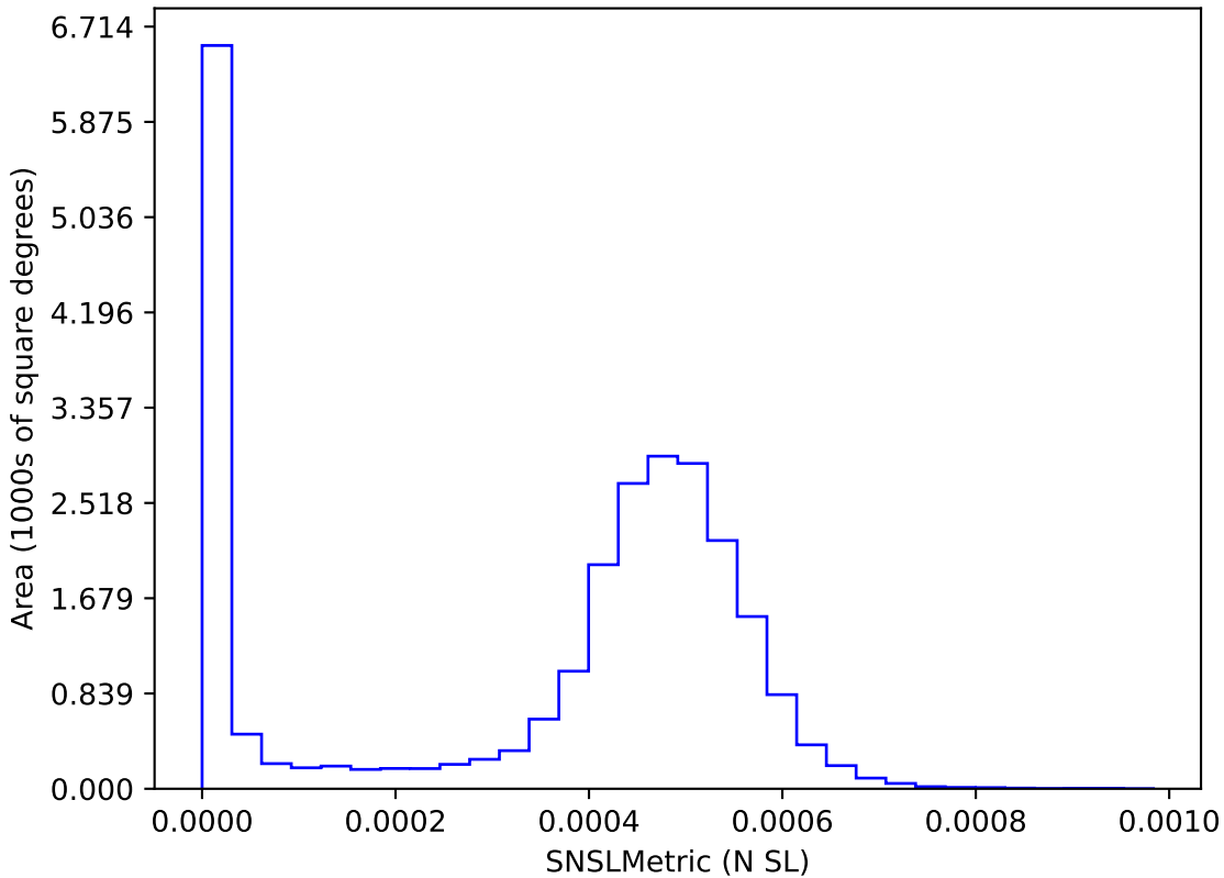
weather_cloudso35v3.4_10yrs : SNSLMetric
