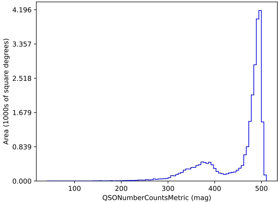
weather_cloudso35v3.4_10yrs z band and non-DD: QSONumberCountsMetric
