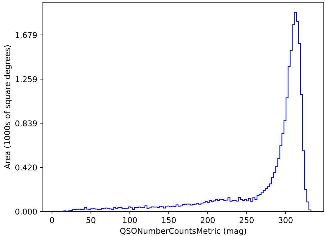
weather_cloudso35v3.4_10yrs u band and non-DD: QSONumberCountsMetric
