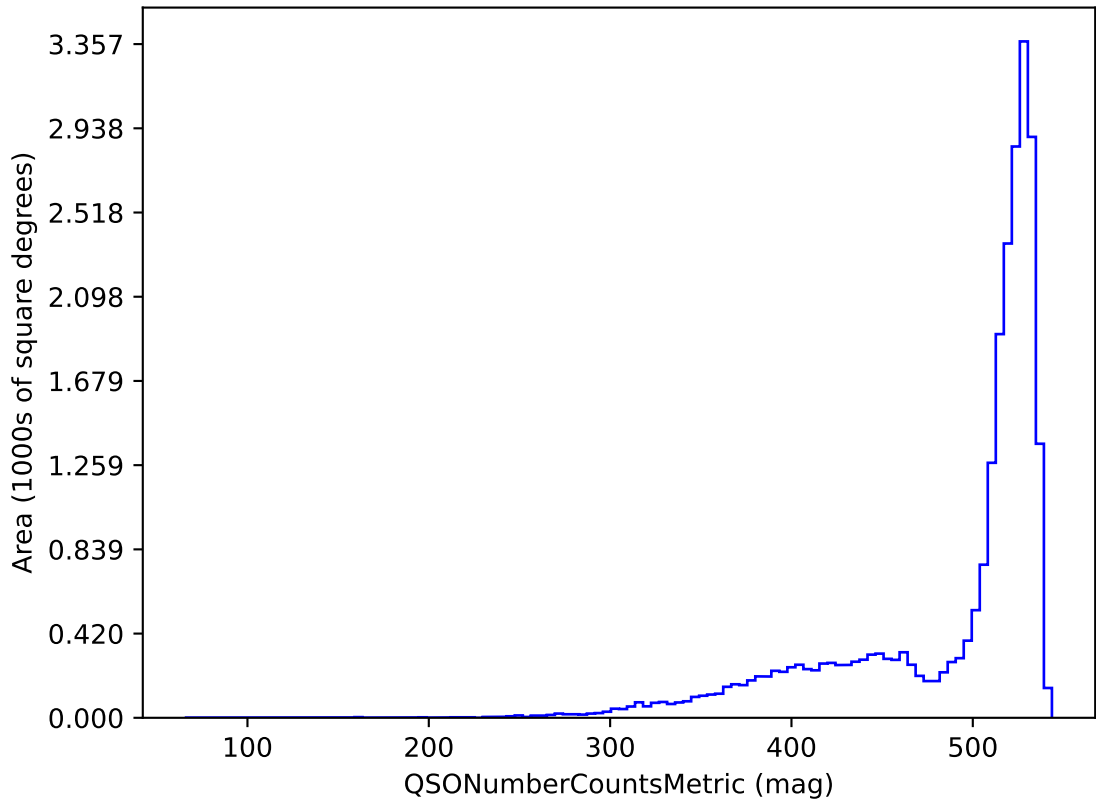
weather_cloudso35v3.4_10yrs r band and non-DD: QSONumberCountsMetric
