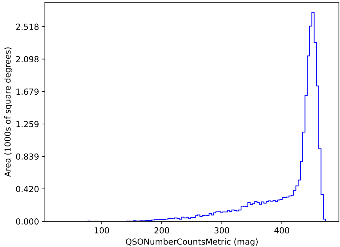
weather_cloudso35v3.4_10yrs g band and non-DD: QSONumberCountsMetric
