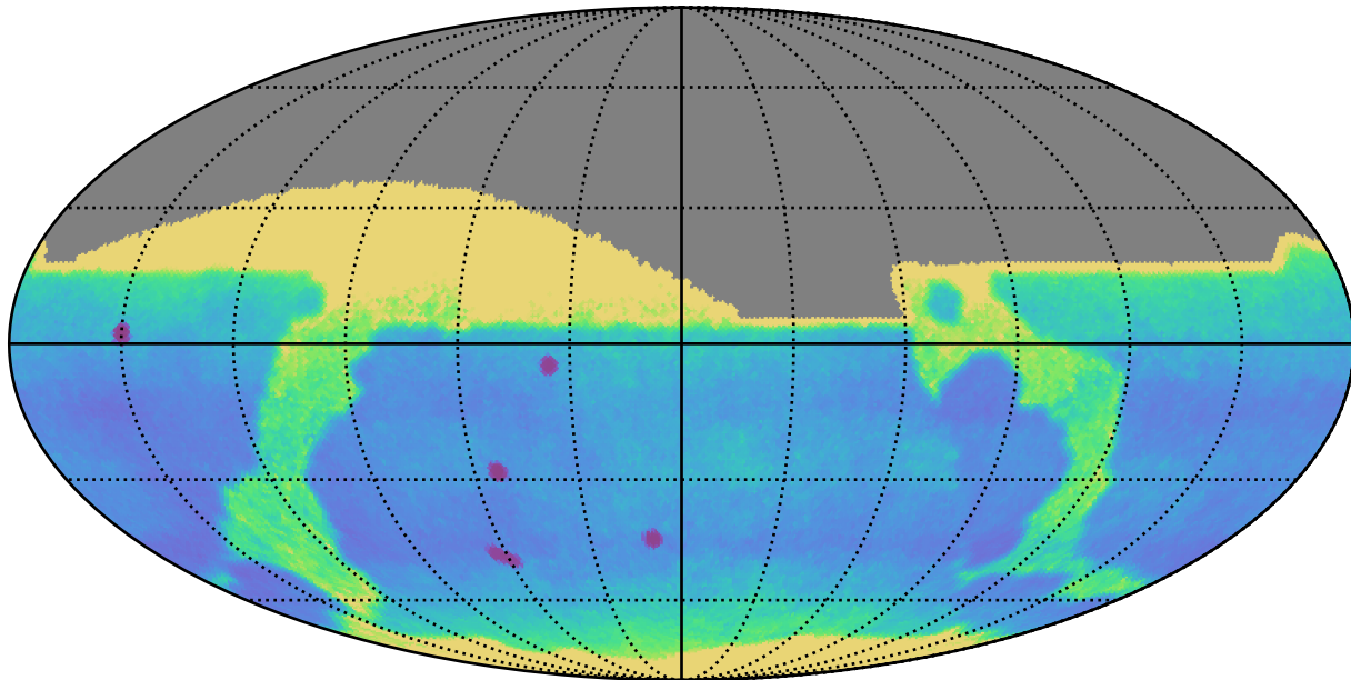
weather_cloudso35v3.4_10yrs : Proper Motion Uncert @ 24.0
