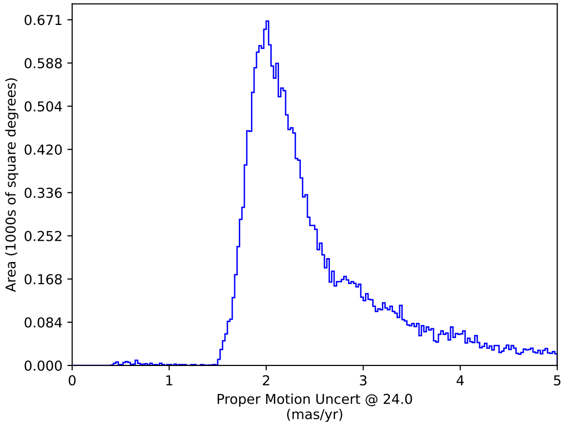
weather_cloudso35v3.4_10yrs : Proper Motion Uncert @ 24.0
