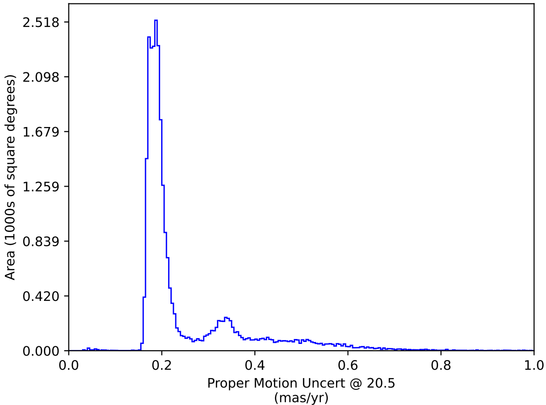
weather_cloudso35v3.4_10yrs : Proper Motion Uncert @ 20.5
