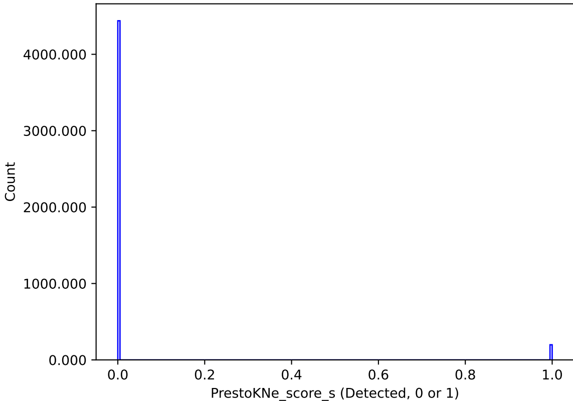
weather_cloudso35v3.4_10yrs : PrestoKNe_score_s
