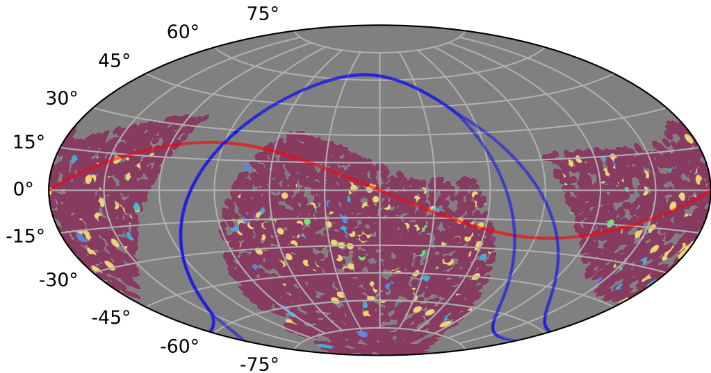
weather_cloudso35v3.4_10yrs : PrestoKNe_score_p
