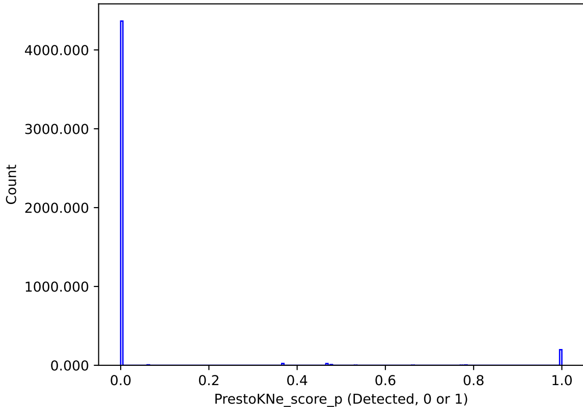
weather_cloudso35v3.4_10yrs : PrestoKNe_score_p
