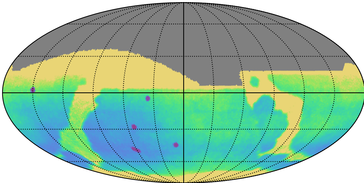
weather_cloudso35v3.4_10yrs : Parallax Uncert @ 24.0
