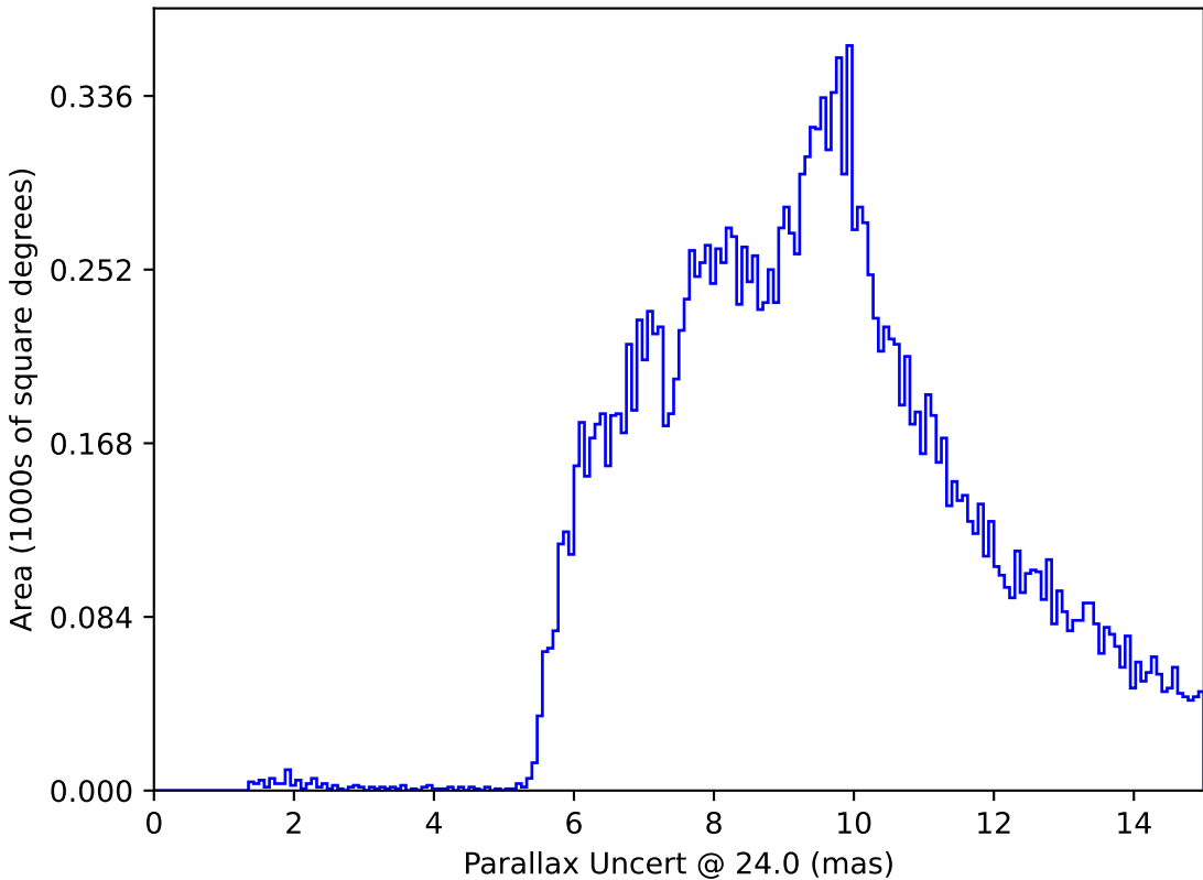
weather_cloudso35v3.4_10yrs : Parallax Uncert @ 24.0
