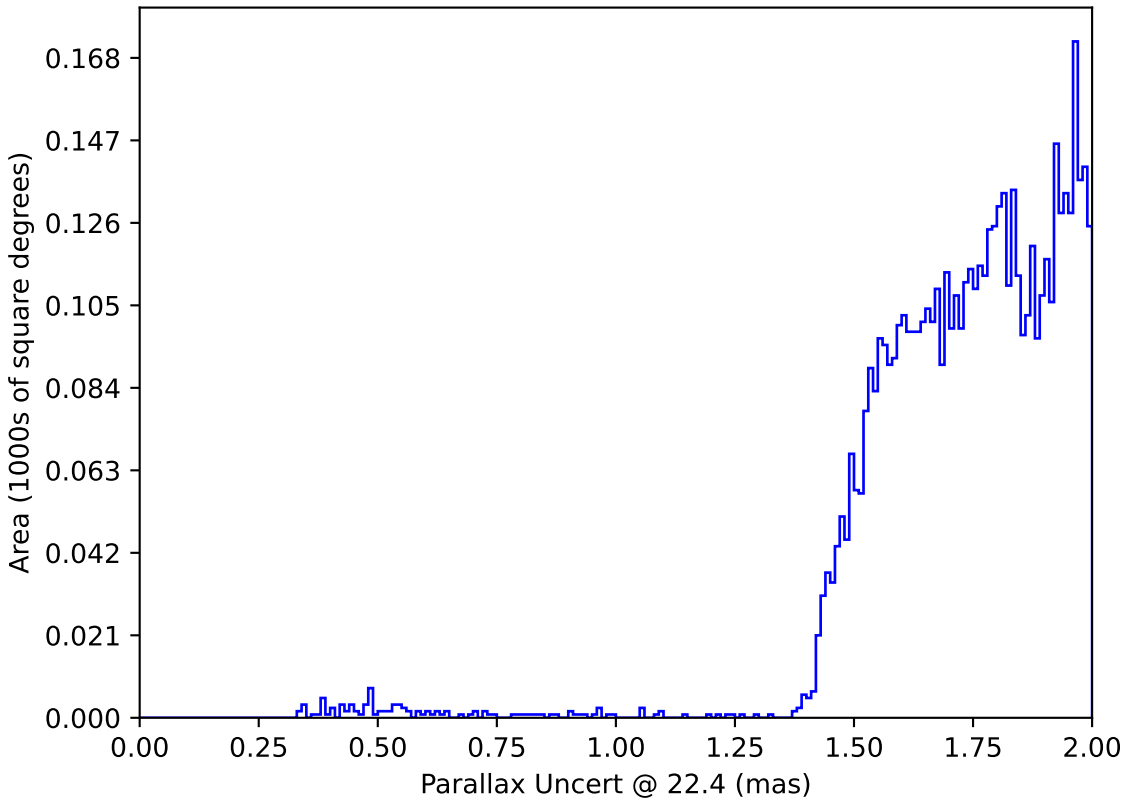
weather_cloudso35v3.4_10yrs : Parallax Uncert @ 22.4
