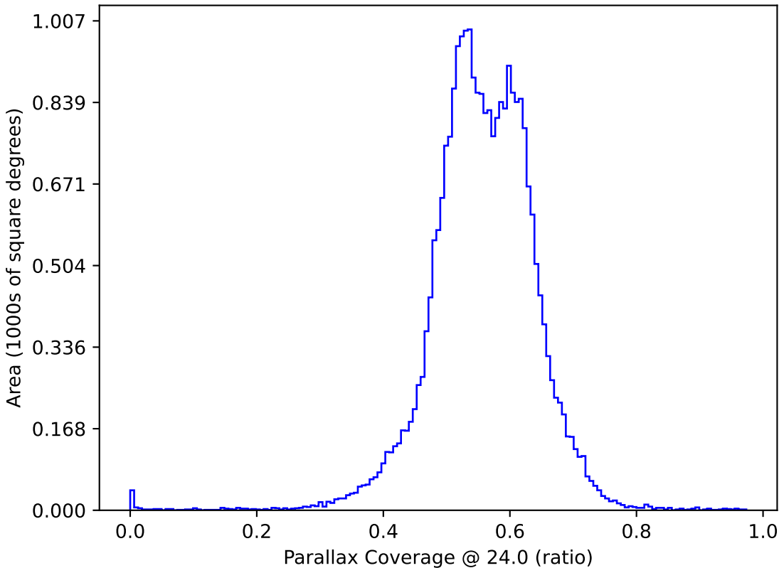
weather_cloudso35v3.4_10yrs : Parallax Coverage @ 24.0
