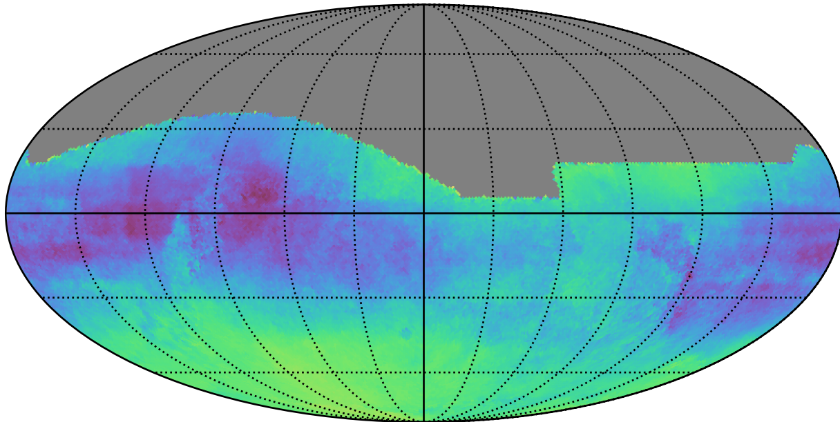
weather_cloudso35v3.4_10yrs : Parallax-DCR degeneracy @ 24.0
